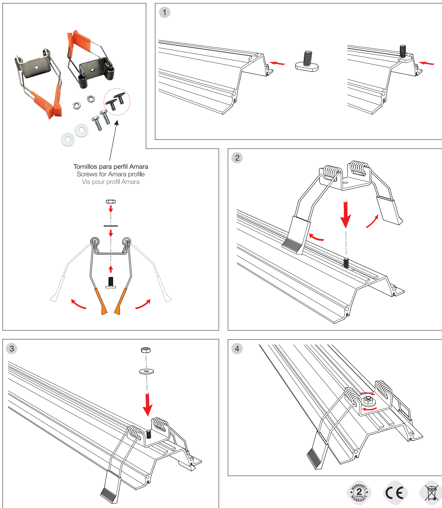
led profile AMARA
